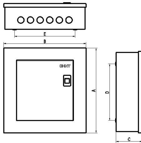
Figure 1 NX6G surface-mounted distribution box
