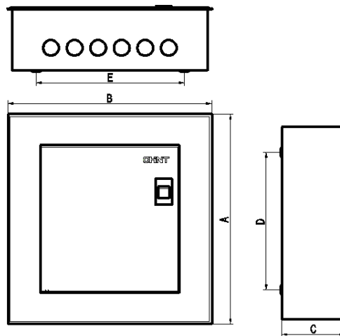
Figure 2 NX6G concealed distribution box
